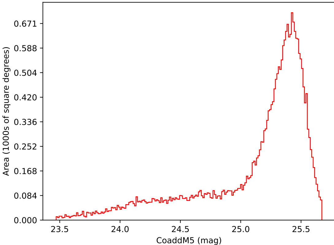
too_elab_r16_d2_giz_v3.4_10yrs Yr 1 i band: CoaddM5
