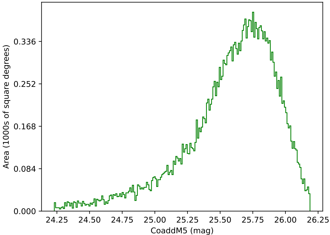
too_elab_r16_d2_giz_v3.4_10yrs Yr 1 g band: CoaddM5
