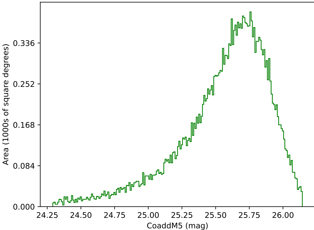
too_elab_r16_d2_giz_v3.4_10yrs Yr 1 g band: CoaddM5
