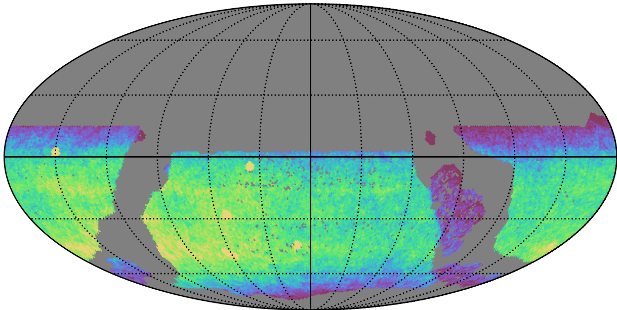
too_elab_r16_d2_giz_v3.4_10yrs WFD y band: CoaddM5
