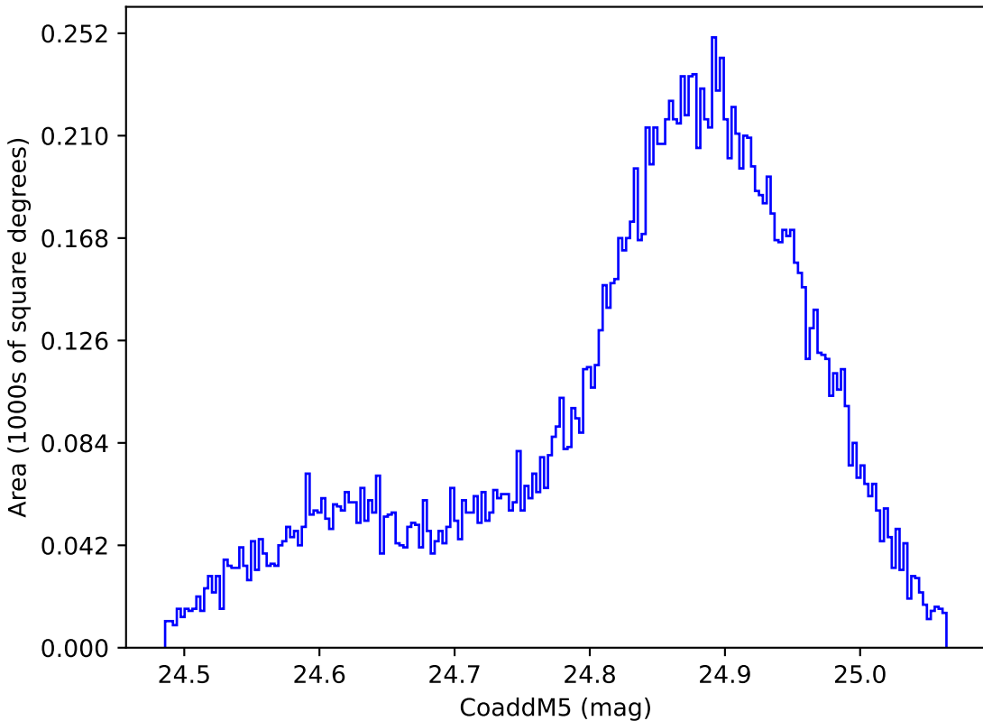
too_elab_r16_d2_giz_v3.4_10yrs WFD y band: CoaddM5
