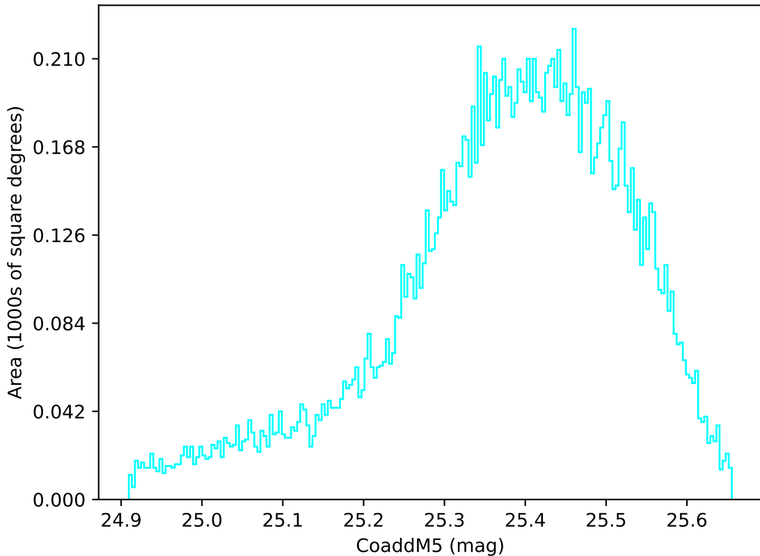
too_elab_r16_d2_giz_v3.4_10yrs WFD u band: CoaddM5
