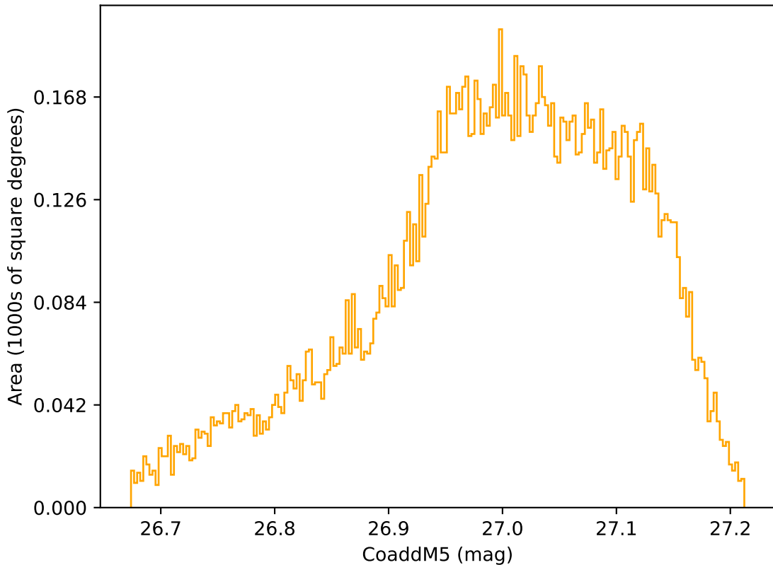
too_elab_r16_d2_giz_v3.4_10yrs WFD r band: CoaddM5
