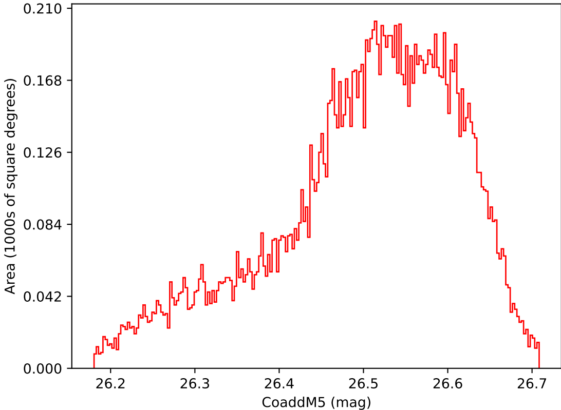
too_elab_r16_d2_giz_v3.4_10yrs WFD i band: CoaddM5
