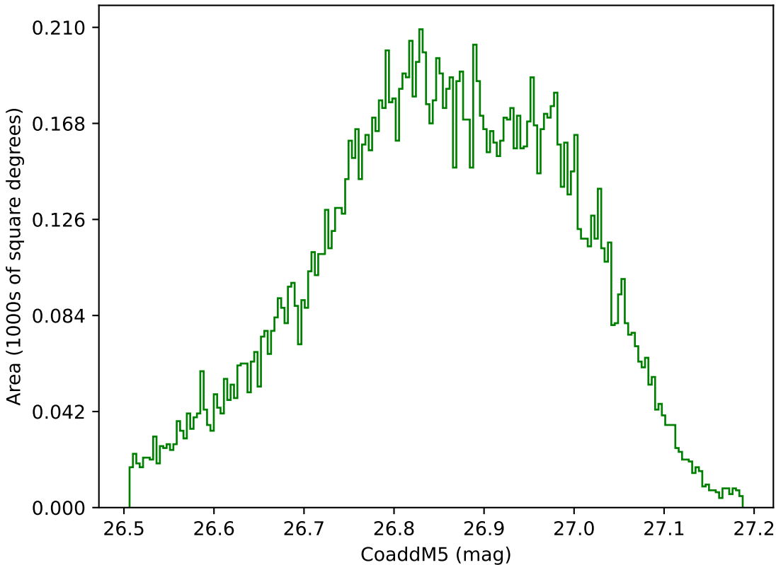
too_elab_r16_d2_giz_v3.4_10yrs WFD g band: CoaddM5
