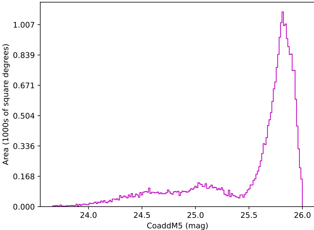
too_elab_r16_d2_giz_v3.4_10yrs All sky z band: CoaddM5
