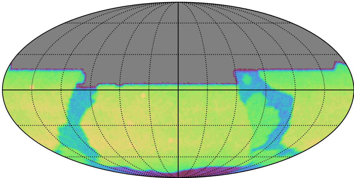
too_elab_r16_d2_giz_v3.4_10yrs All sky y band: CoaddM5
