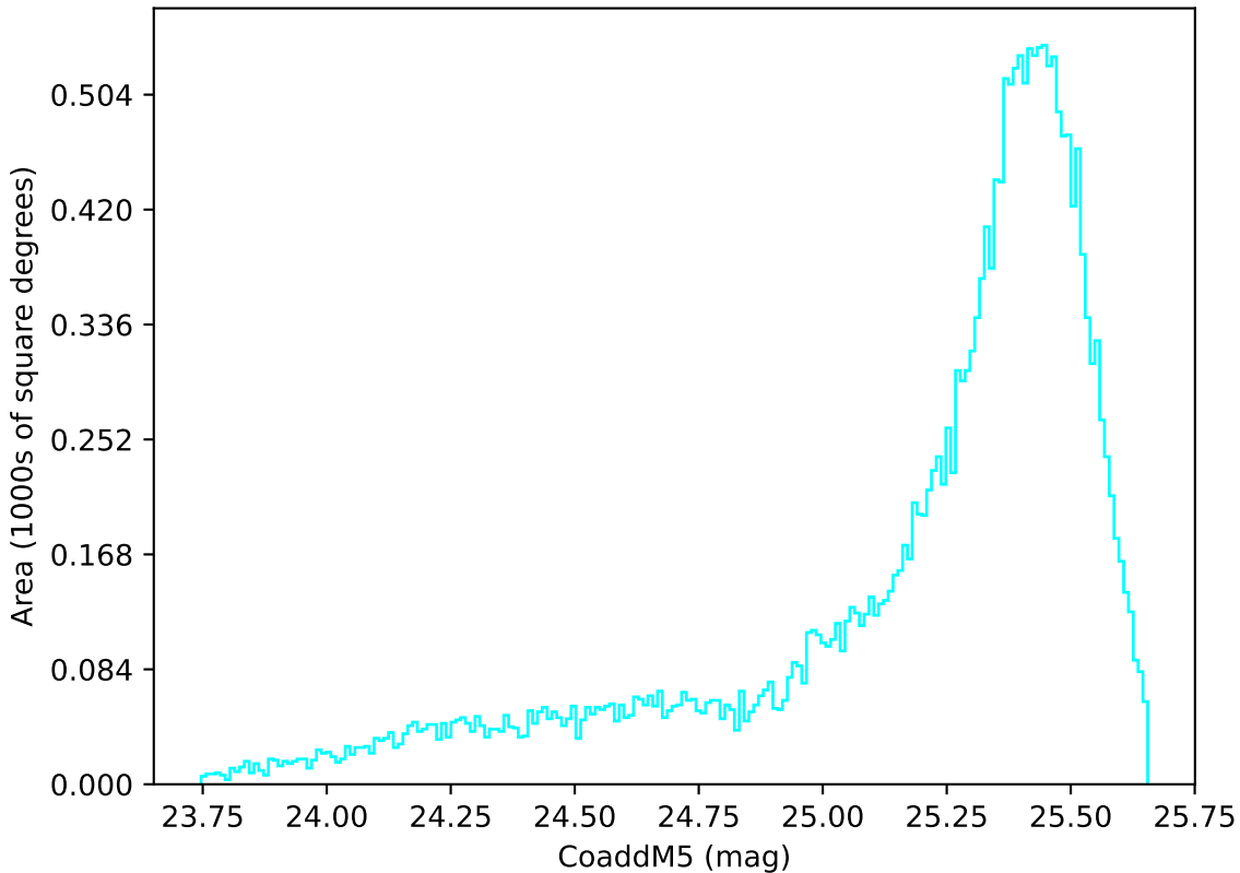
too_elab_r16_d2_giz_v3.4_10yrs All sky u band: CoaddM5
