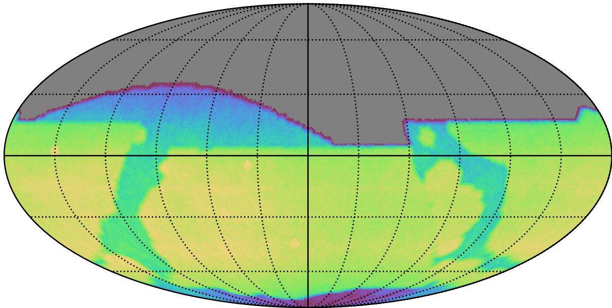
too_elab_r16_d2_giz_v3.4_10yrs All sky r band: CoaddM5
