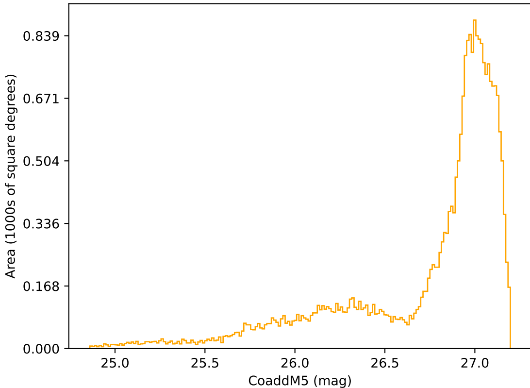
too_elab_r16_d2_giz_v3.4_10yrs All sky r band: CoaddM5
