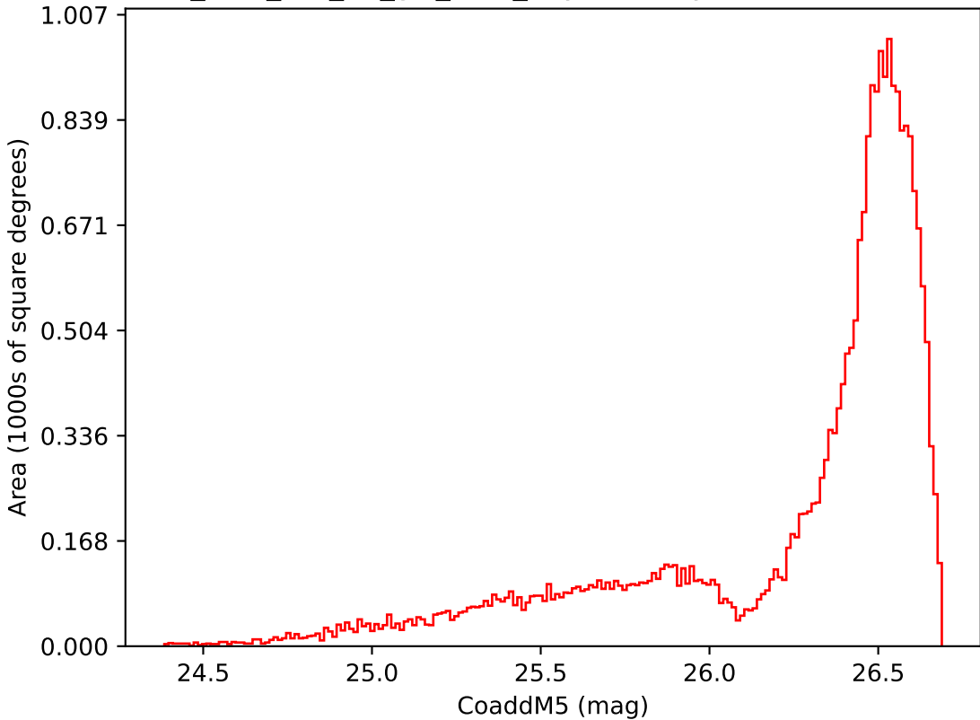
too_elab_r16_d2_giz_v3.4_10yrs All sky i band: CoaddM5
