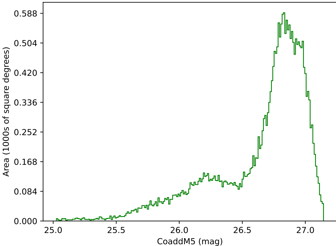
too_elab_r16_d2_giz_v3.4_10yrs All sky g band: CoaddM5
