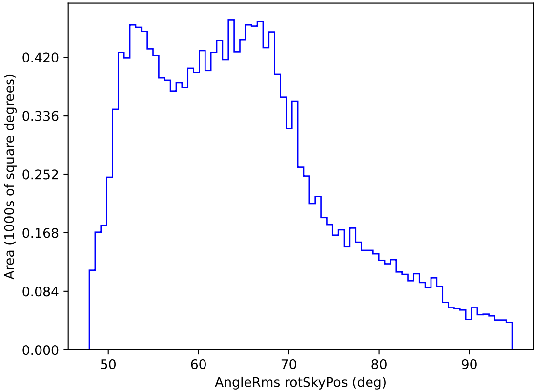
too_elab_r16_d2_giz_v3.4_10yrs WFD z band: AngleRms rotSkyPos
