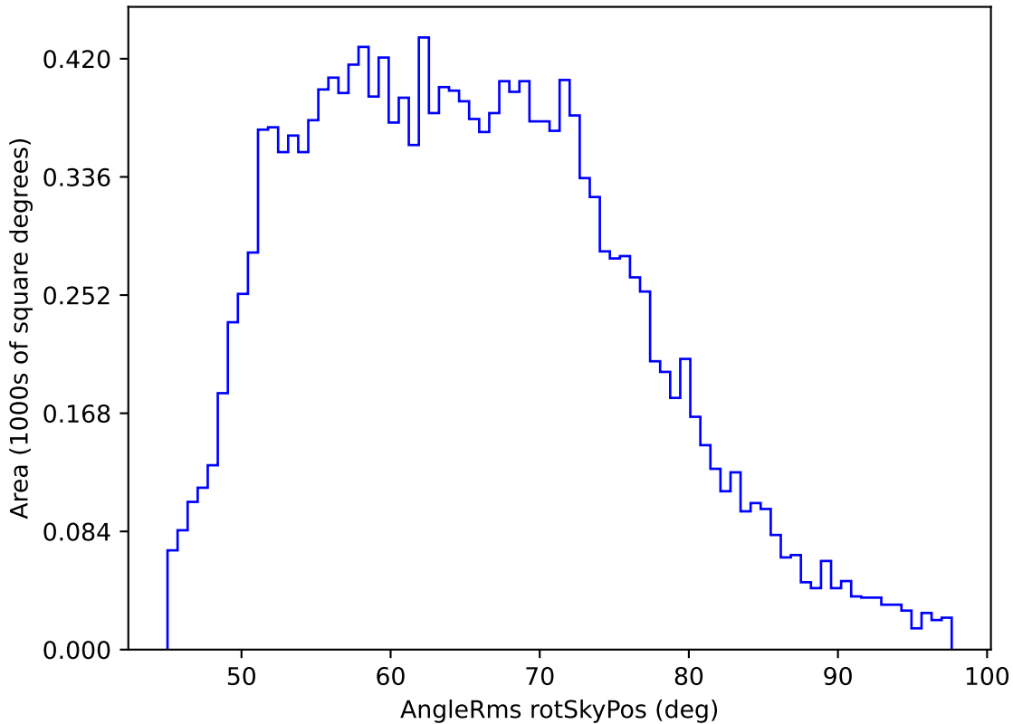
too_elab_r16_d2_giz_v3.4_10yrs WFD u band: AngleRms rotSkyPos
