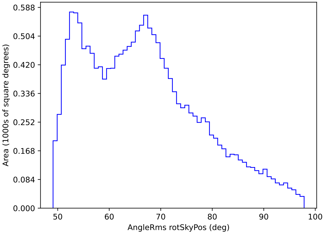
too_elab_r16_d2_giz_v3.4_10yrs WFD r band: AngleRms rotSkyPos
