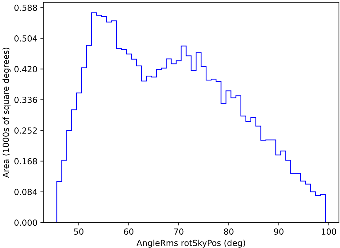
too_elab_r16_d2_giz_v3.4_10yrs WFD g band: AngleRms rotSkyPos
