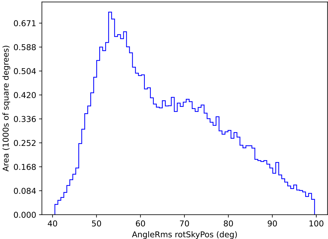
too_elab_r16_d2_giz_v3.4_10yrs All sky g band: AngleRms rotSkyPos
