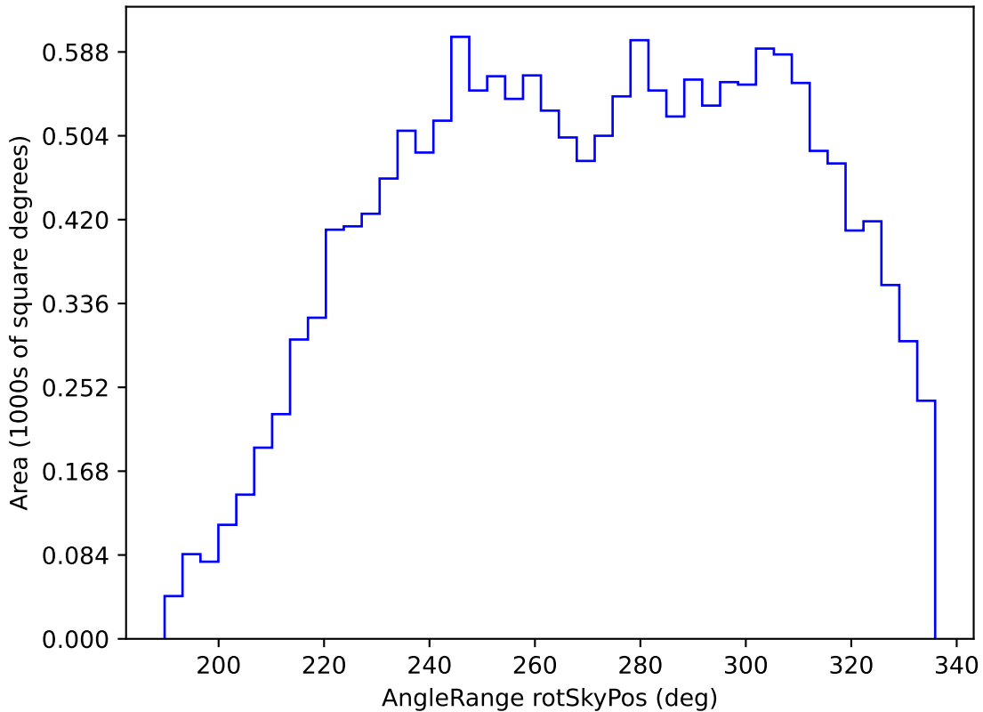
too_elab_r16_d2_giz_v3.4_10yrs WFD y band: AngleRange rotSkyPos
