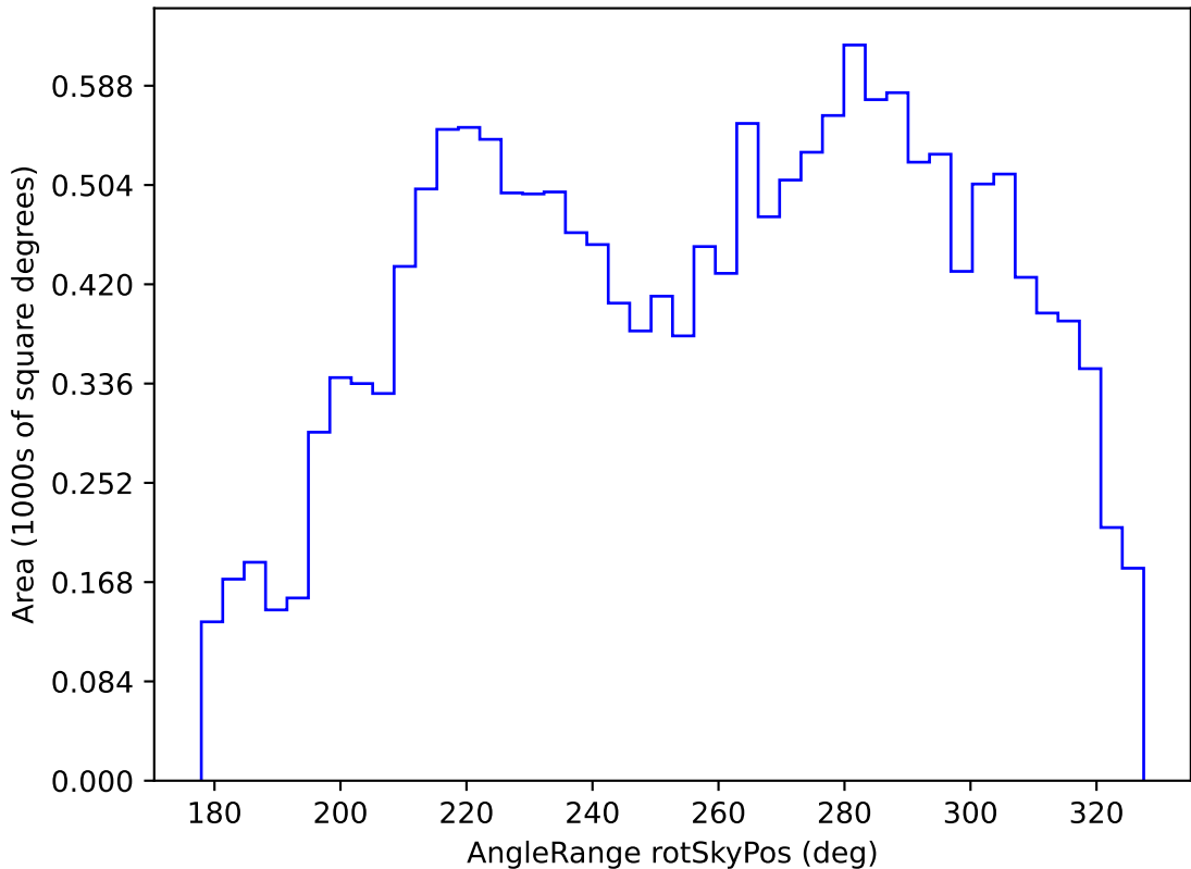
too_elab_r16_d2_giz_v3.4_10yrs WFD u band: AngleRange rotSkyPos
