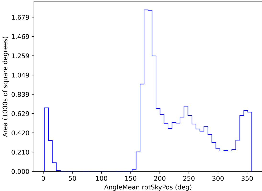
too_elab_r16_d2_giz_v3.4_10yrs WFD y band: AngleMean rotSkyPos
