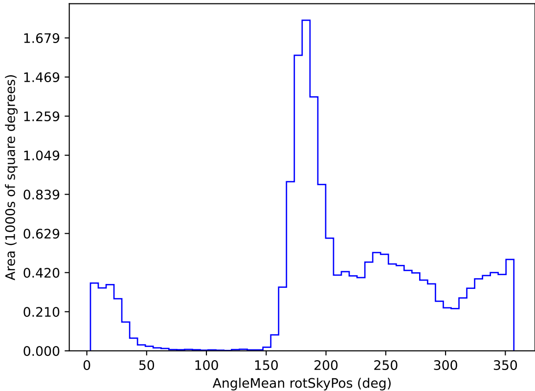
too_elab_r16_d2_giz_v3.4_10yrs WFD u band: AngleMean rotSkyPos
