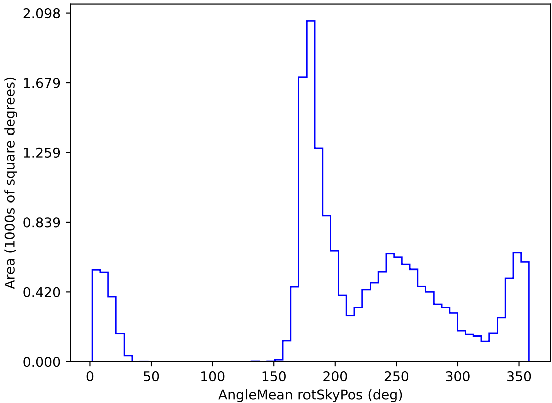
too_elab_r16_d2_giz_v3.4_10yrs WFD i band: AngleMean rotSkyPos
