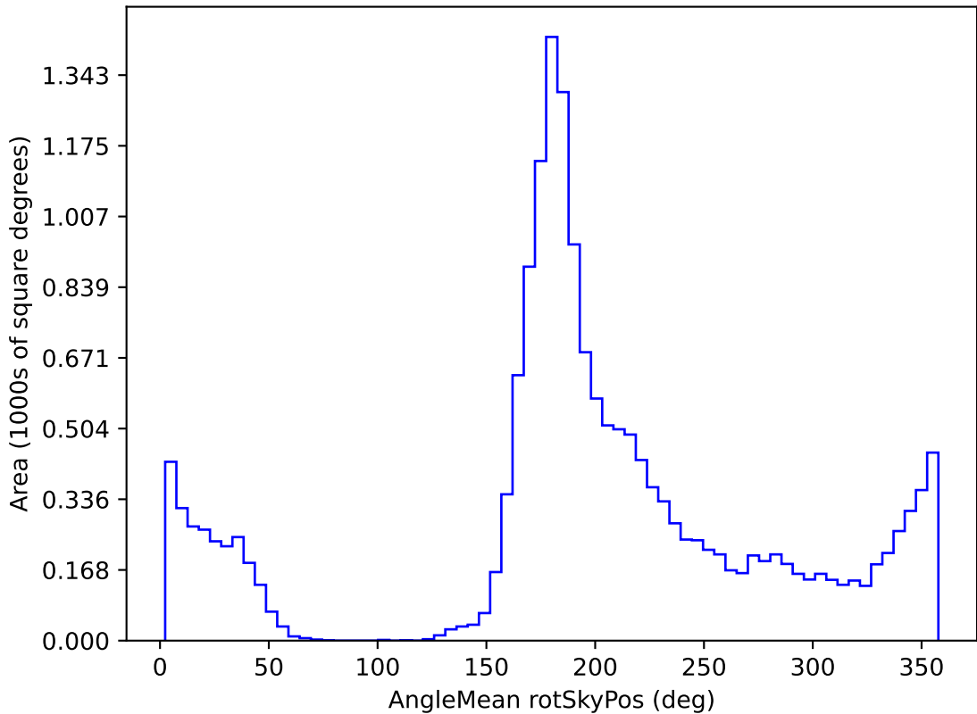
too_elab_r16_d2_giz_v3.4_10yrs WFD g band: AngleMean rotSkyPos
