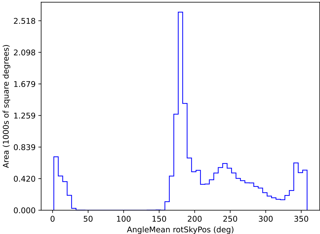
too_elab_r16_d2_giz_v3.4_10yrs WFD all bands: AngleMean rotSkyPos
