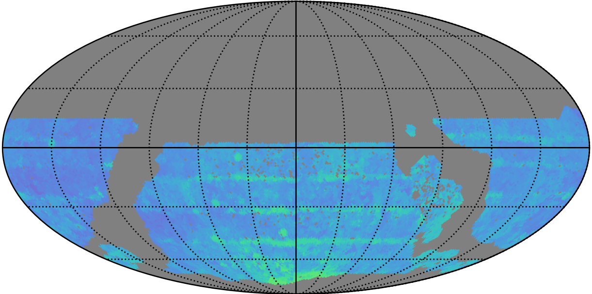
too_elab_r16_d2_giz_v3.4_10yrs WFD z band: 80thPercentile Season Length
