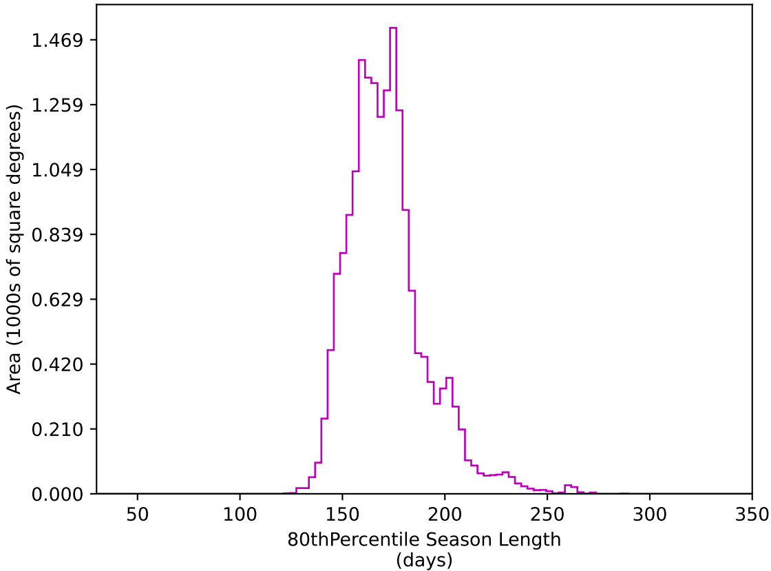
too_elab_r16_d2_giz_v3.4_10yrs WFD z band: 80thPercentile Season Length
