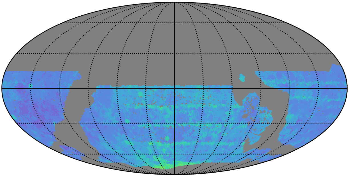
too_elab_r16_d2_giz_v3.4_10yrs WFD y band: 80thPercentile Season Length
