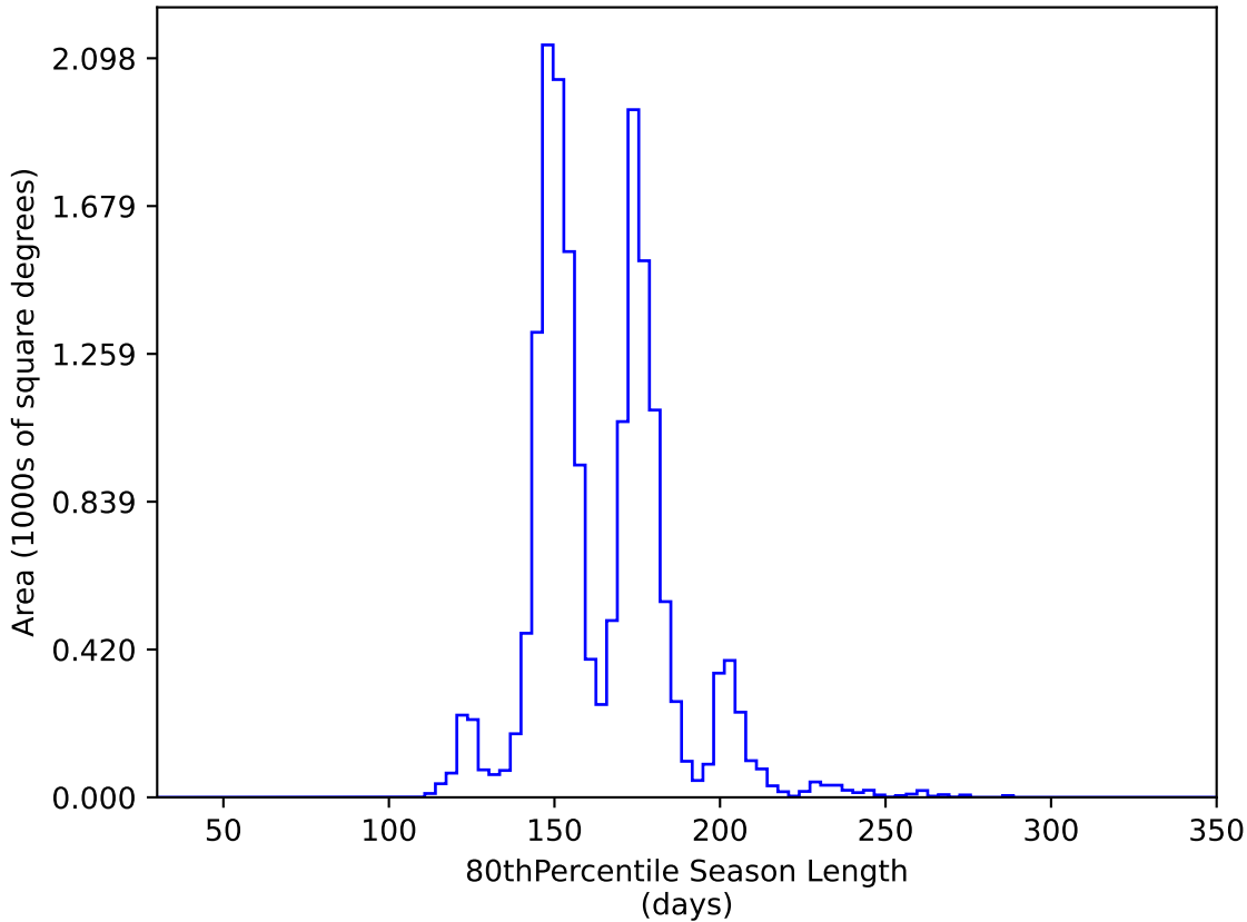
too_elab_r16_d2_giz_v3.4_10yrs WFD y band: 80thPercentile Season Length
