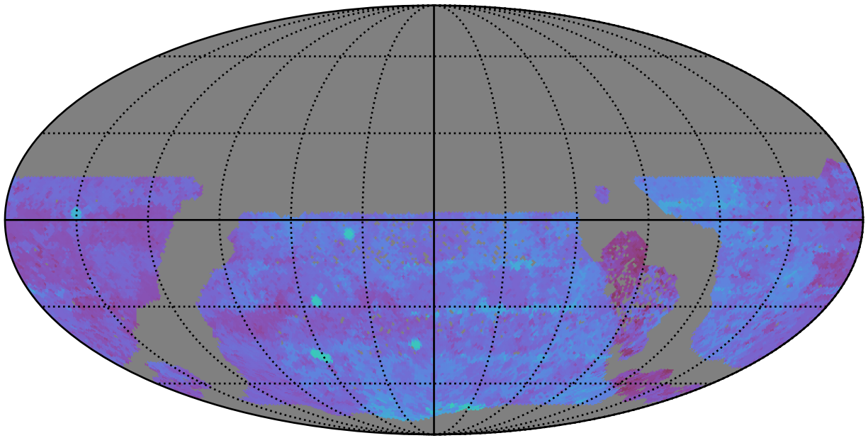
too_elab_r16_d2_giz_v3.4_10yrs WFD u band: 80thPercentile Season Length
