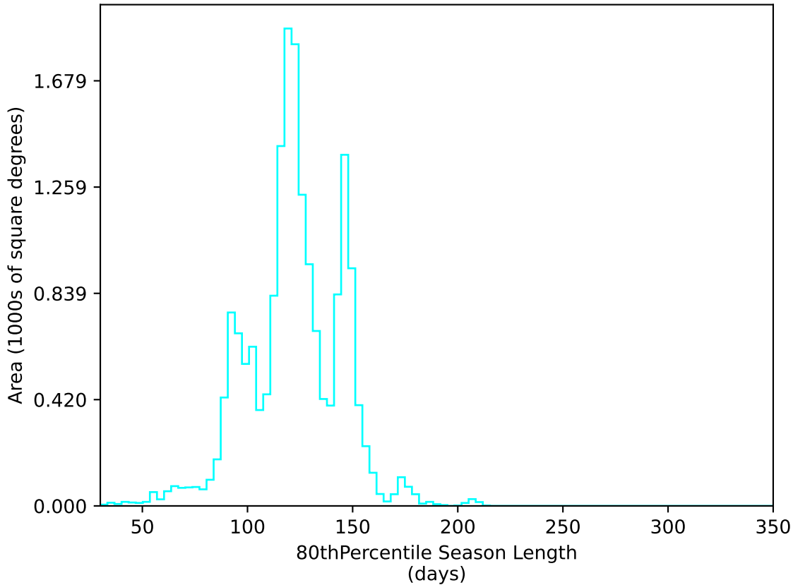
too_elab_r16_d2_giz_v3.4_10yrs WFD u band: 80thPercentile Season Length
