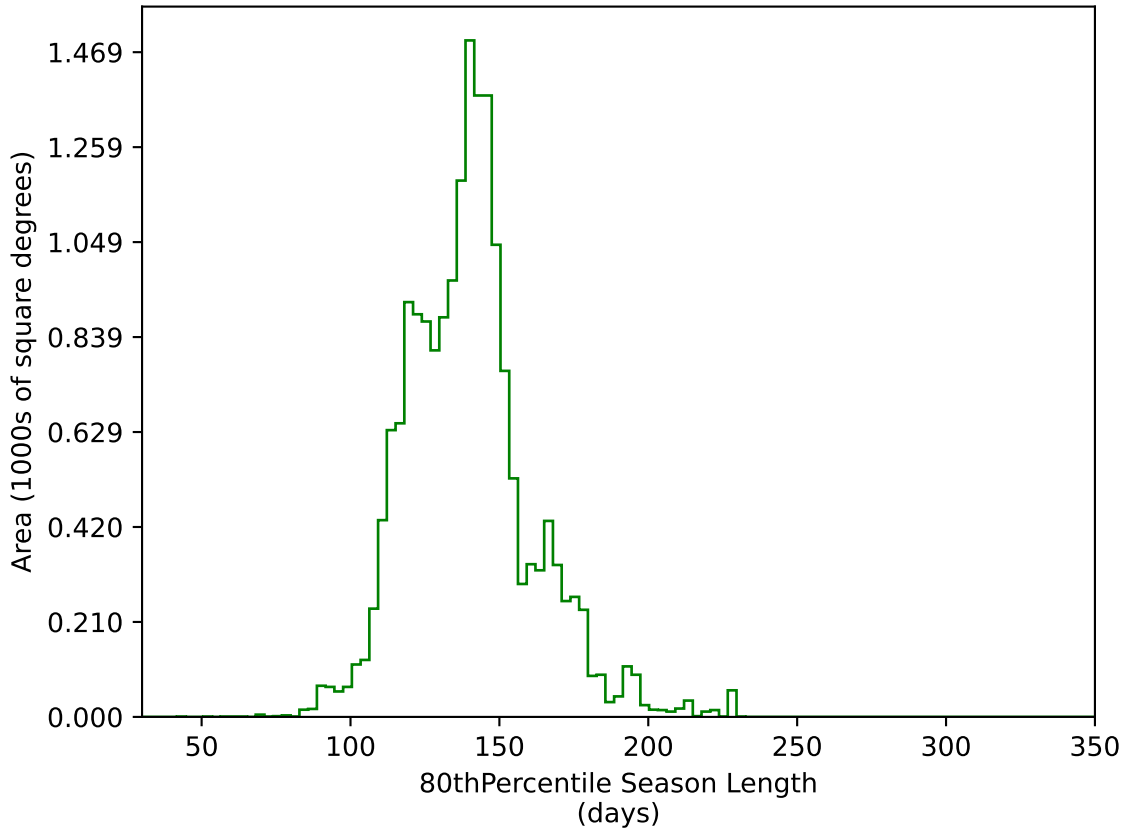
too_elab_r16_d2_giz_v3.4_10yrs WFD g band: 80thPercentile Season Length
