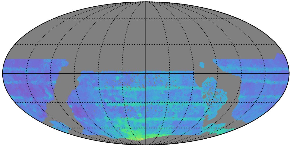
too_elab_r16_d2_giz_v3.4_10yrs WFD all bands: 80thPercentile Season Length
