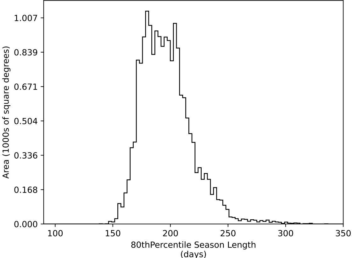
too_elab_r16_d2_giz_v3.4_10yrs WFD all bands: 80thPercentile Season Length
