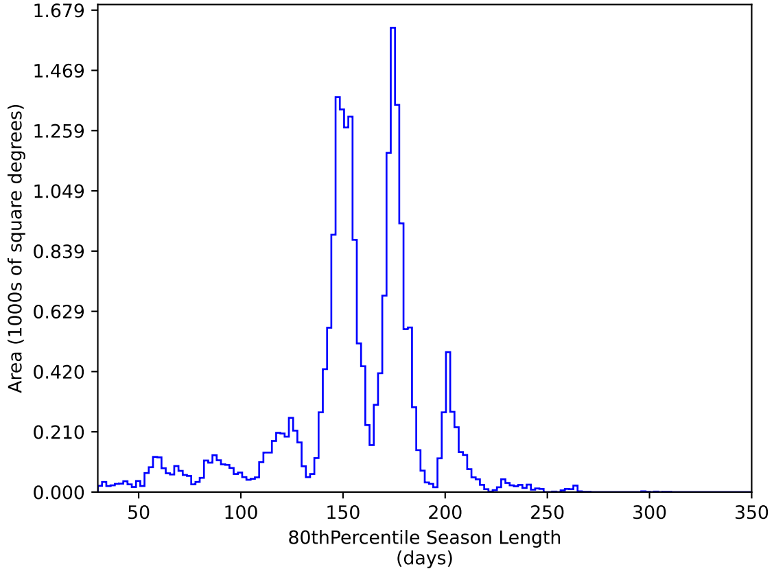
too_elab_r16_d2_giz_v3.4_10yrs All sky y band: 80thPercentile Season Length
