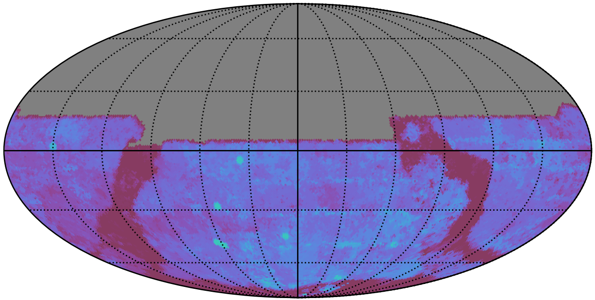
too_elab_r16_d2_giz_v3.4_10yrs All sky u band: 80thPercentile Season Length
