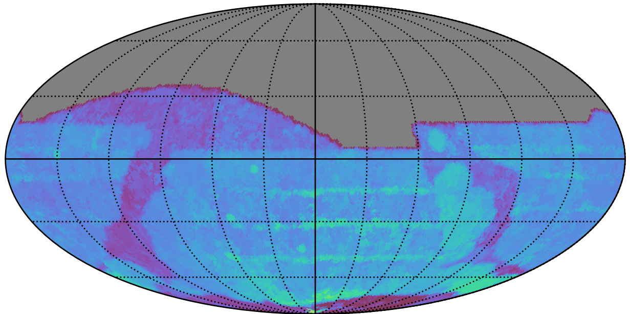
too_elab_r16_d2_giz_v3.4_10yrs All sky r band: 80thPercentile Season Length
