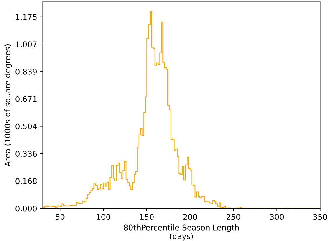
too_elab_r16_d2_giz_v3.4_10yrs All sky r band: 80thPercentile Season Length
