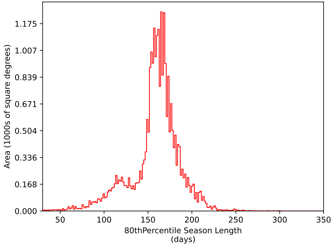
too_elab_r16_d2_giz_v3.4_10yrs All sky i band: 80thPercentile Season Length
