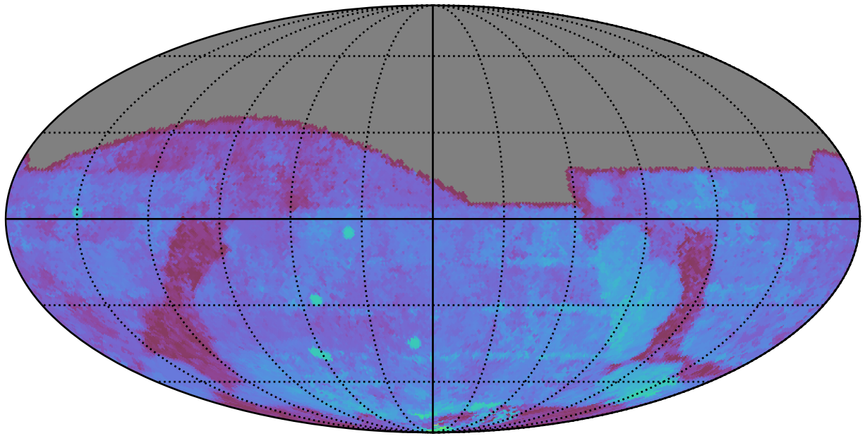
too_elab_r16_d2_giz_v3.4_10yrs All sky g band: 80thPercentile Season Length
