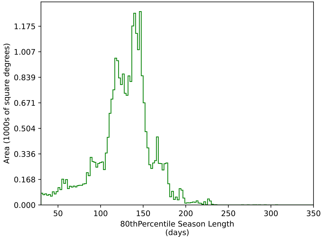
too_elab_r16_d2_giz_v3.4_10yrs All sky g band: 80thPercentile Season Length
