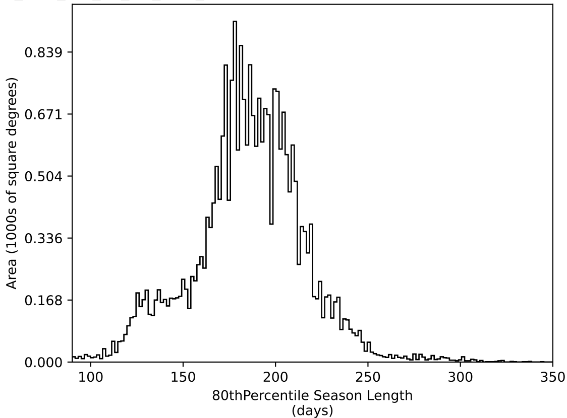
too_elab_r16_d2_giz_v3.4_10yrs All sky all bands: 80thPercentile Season Length
