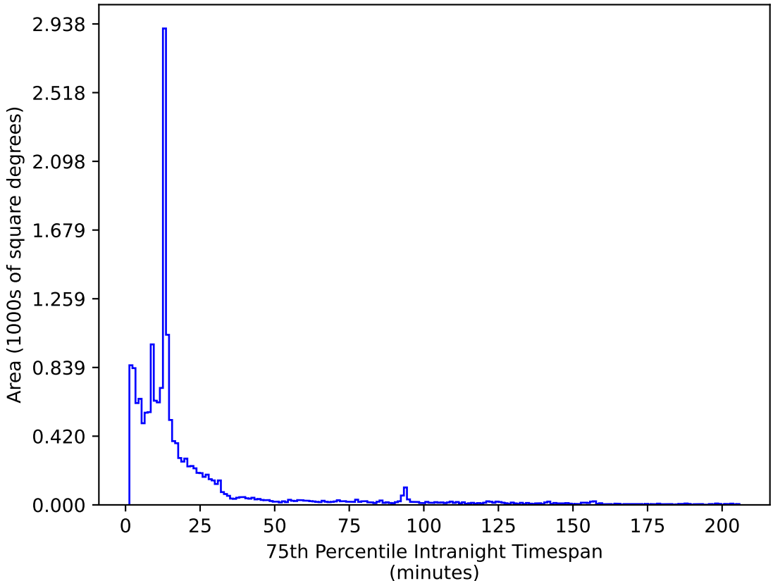
too_elab_r16_d2_giz_v3.4_10yrs WFD z band: 75th Percentile Intranight Timespan
