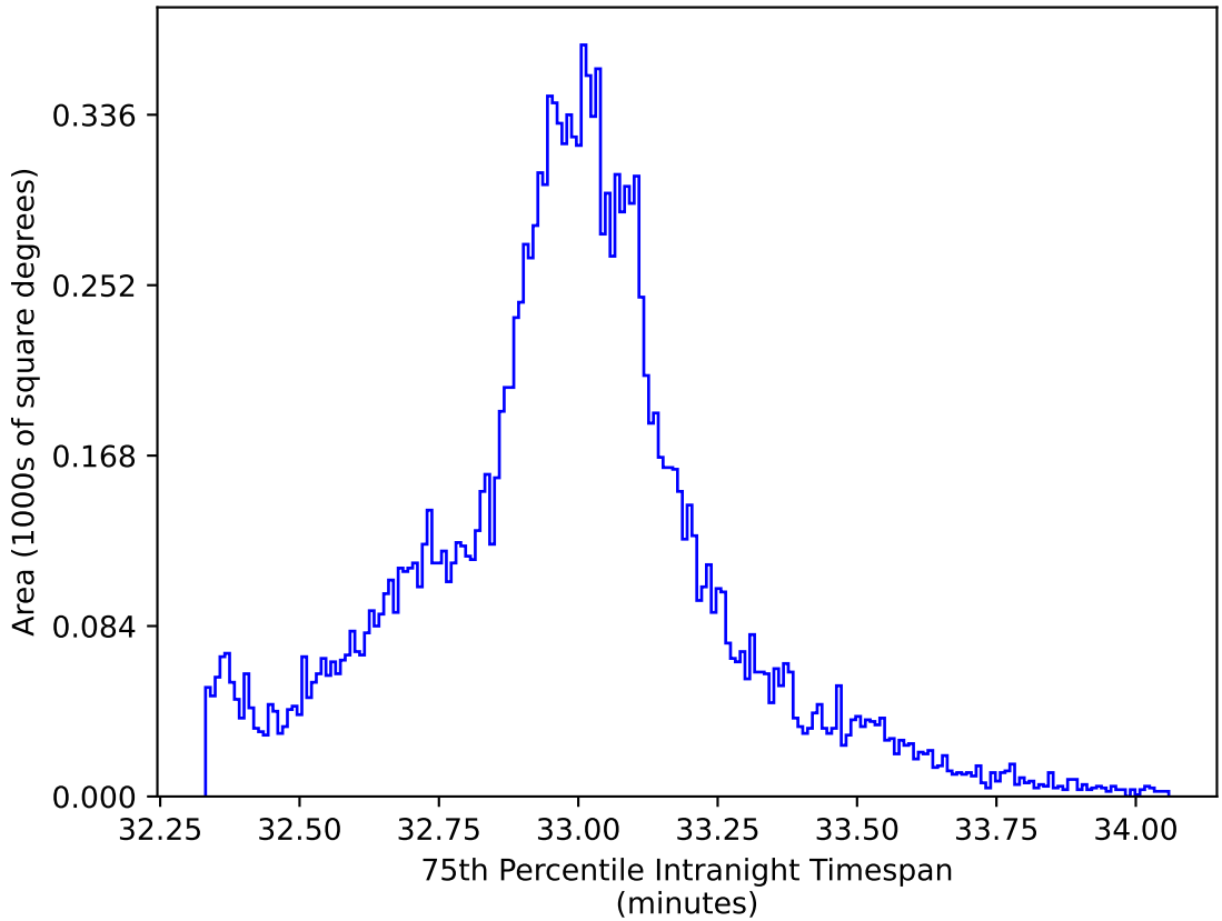
too_elab_r16_d2_giz_v3.4_10yrs WFD y band: 75th Percentile Intranight Timespan
