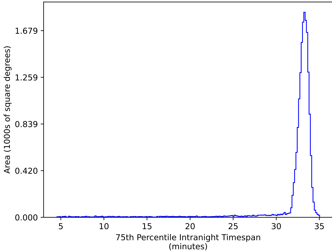
too_elab_r16_d2_giz_v3.4_10yrs WFD ug bands: 75th Percentile Intranight Timespan
