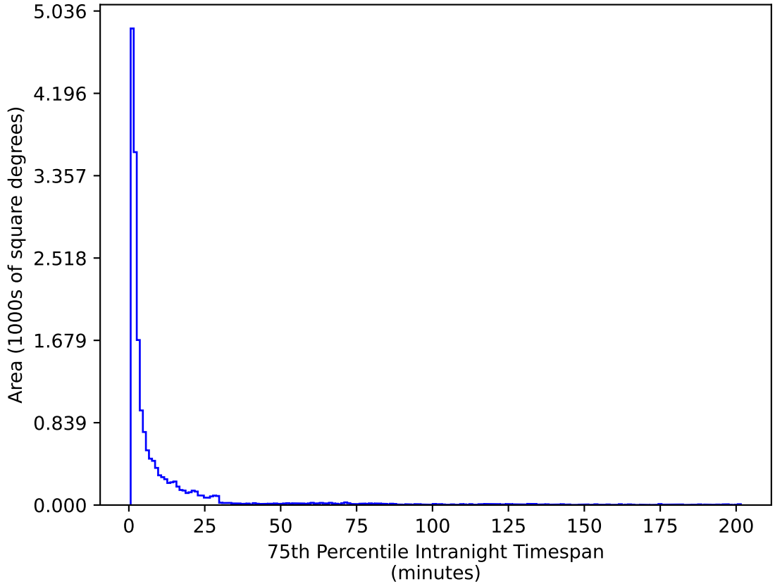
too_elab_r16_d2_giz_v3.4_10yrs WFD u band: 75th Percentile Intranight Timespan
