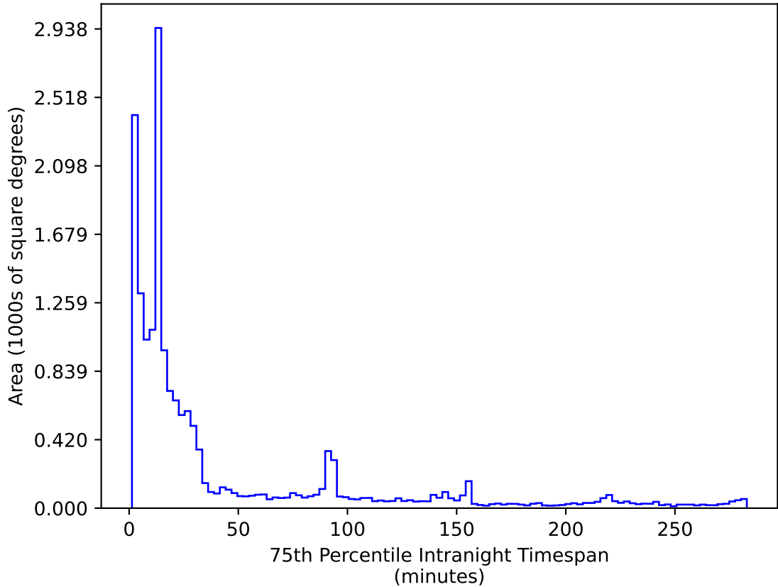
too_elab_r16_d2_giz_v3.4_10yrs WFD r band: 75th Percentile Intranight Timespan
