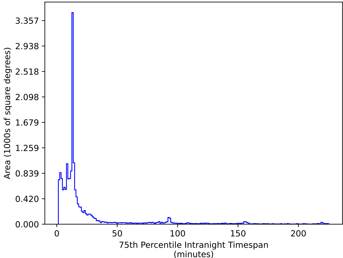
too_elab_r16_d2_giz_v3.4_10yrs WFD i band: 75th Percentile Intranight Timespan
